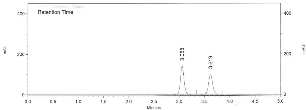
Figure 11 : Linearity results of level 50
